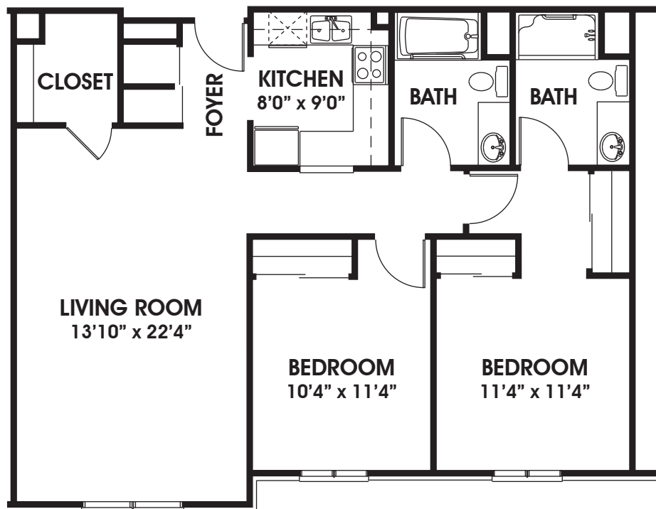
DOROTHY LOVE APARTMENTS TWO BEDROOM STANDARD UNIT 1023 S.F.
